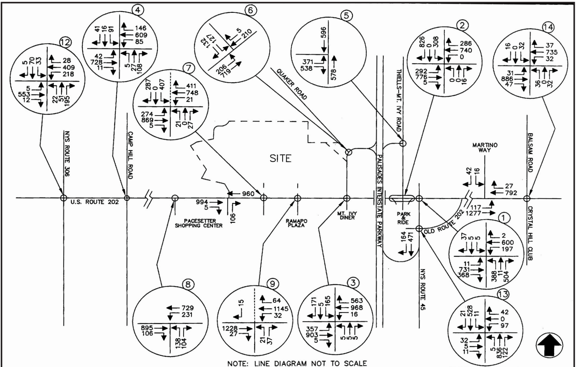
Figure 3.5-25: 2011 Build Traffic Volumes Weekday Peak PM Highway Hour (W/O Patrick Farm) Minisceongo Park Towns of Haverstraw & Ramapo, Rockland County, New York Source: John Collins Engineers, P.C. Date: October, 2008
